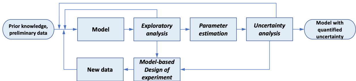
Fig. 17.1: Pyomo.DoE integrates exploratory analysis, parameter estimation, uncertainty analysis, and MBDoE into an iterative framework to select, refine, and calibrate science-based mathematical models with quantified uncertainty. Currently, Pyomo.DoE focuses on increasing parameter precision.
